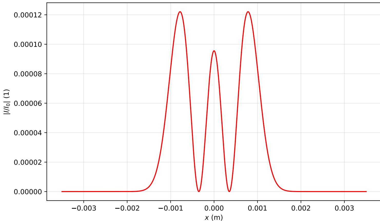
Intensity profile I(x, y = 0, z = 0.080)/I_0 , \text{Pin}=9.0\text{Pcr} , artificial time
